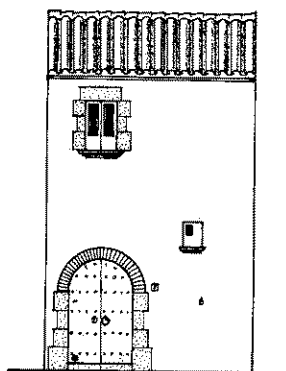
FAÇANA PRINCIPAL
