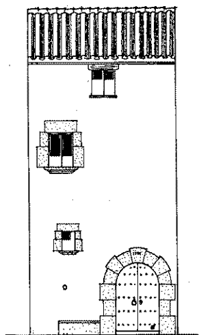
FAÇANA PRINCIPAL
